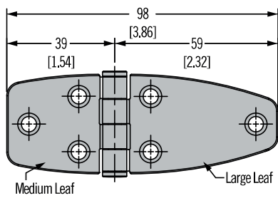
Style 6 (Part Number see table)
